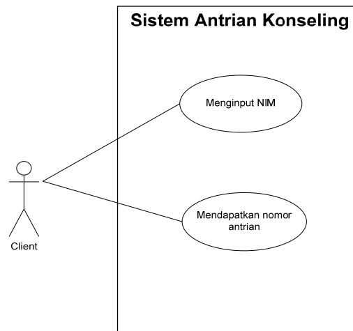
Gambar 2 Use Case Sisi Client
